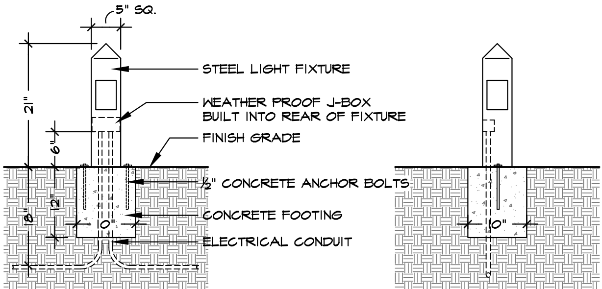
FRONT VIEW
